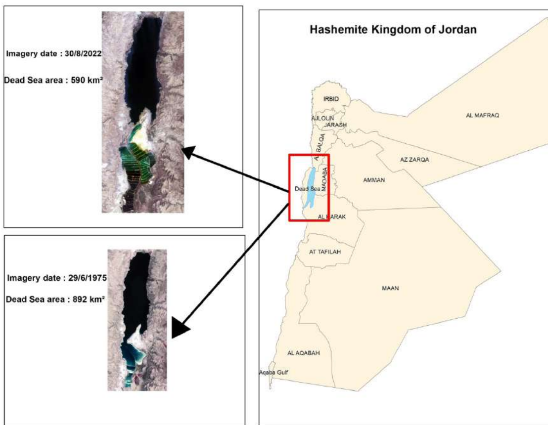
Fig.2 : Dead Sea area in 1975 & 2022
